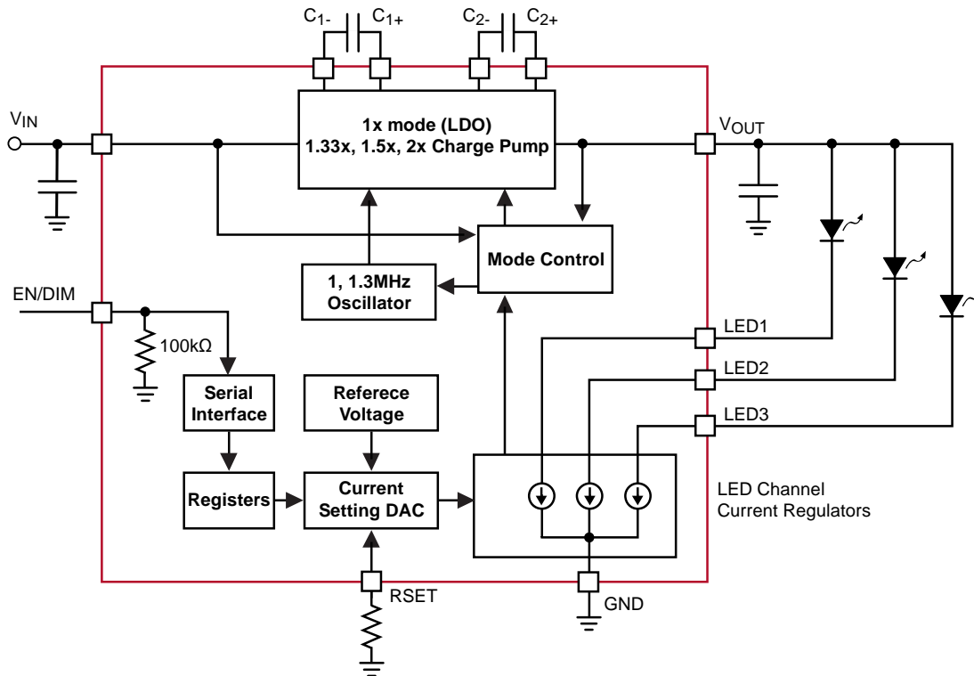
Figure 2. SET3643 Functional Block Diagram
