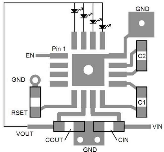
Figure 4. PCB Layout
