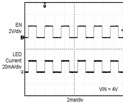
300Hz PWM waveform (1x mode)
