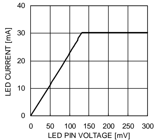
LED Current vs. LED Pin Voltage
