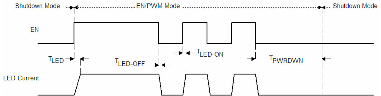
Figure 1. SET3604V Timing Characteristics
