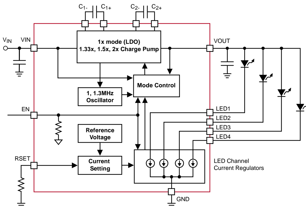
Figure 2. SET3604V Functional Block Diagram
